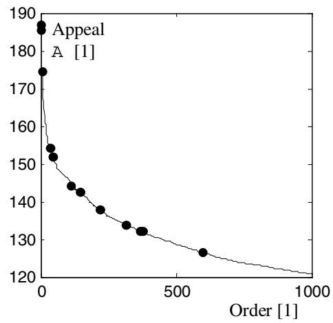
Fig. 3. The sequence of the largest values of appeal A ; cases selected for the basis (see Fig. 4 by rows).
