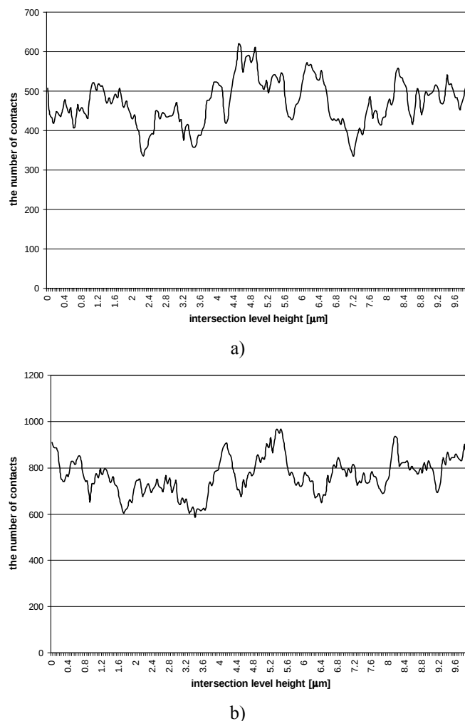
Fig 3. Generated curves for the contact surfaces number through the intersection planes of the BaTiO 3 -ceramic sample system with: a) 500 grains and b) 700 grains.
