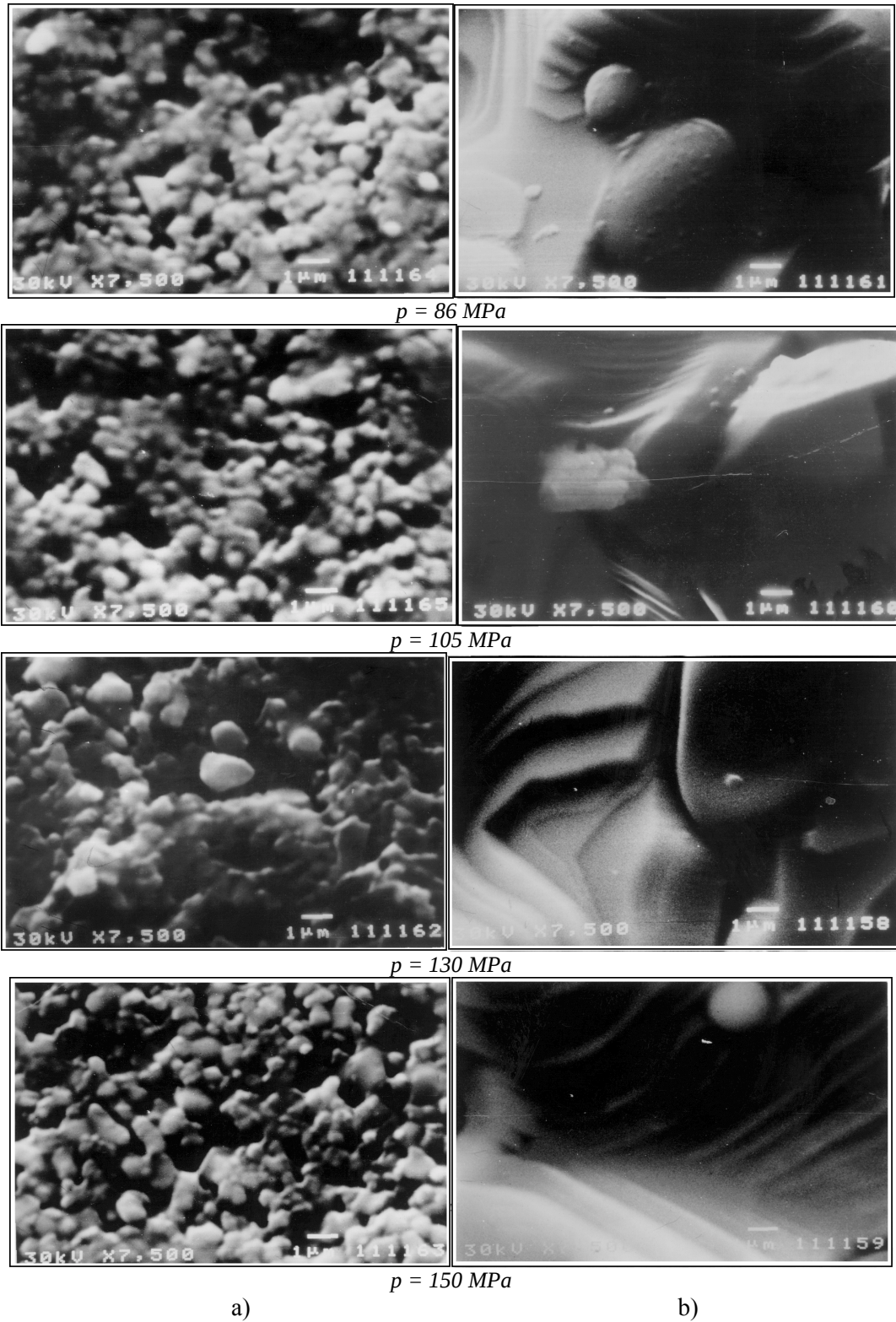
Fig. 1. SEM microphotographs of BaTiO 3 -ceramic samples: a) pressed samples; b) sintered samples ( T_{\text{sint}} = 1370^\circ\text{C} , \tau_{\text{sint}} = 2\text{h} ) ( \times 7500 ).
